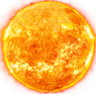
Slunce
