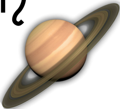
Saturn
